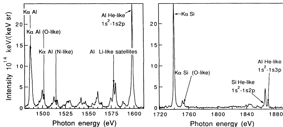
FIG. 1. Spectra obtained with 500 \text{\AA} Al thickness on a \text{SiO}_2 substrate at a laser intensity of 3 \times 10^{16} W/cm 2 . Left: emission from aluminum plasma. Right: emission from silicon plasma.
